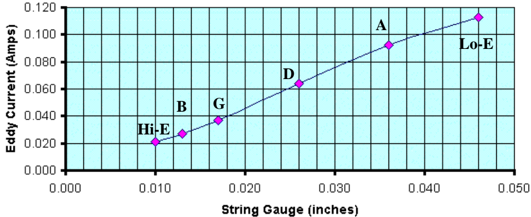
Eddy Current vs. String Gauge
