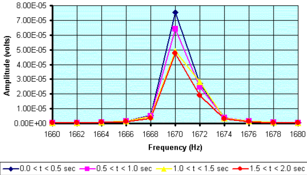
Amplitude vs. Frequency of Vibrating Rod Fundamental Mode @ f_1 = 1670 Hz
